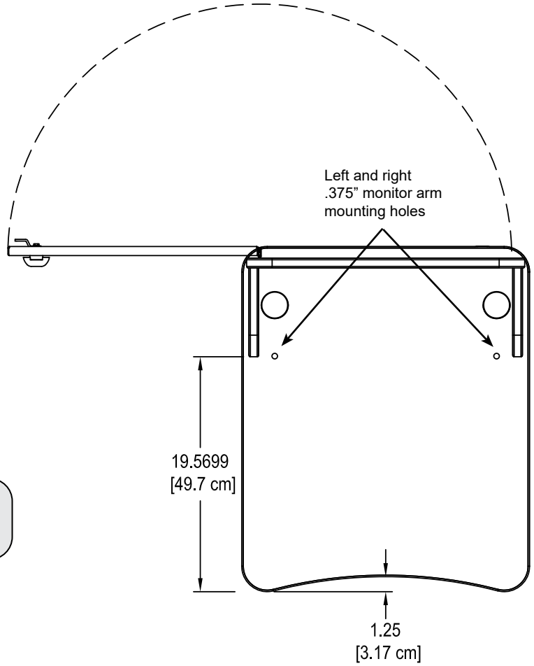
42" Inspiration Plus Lectern with 5" Balloon Wheels
