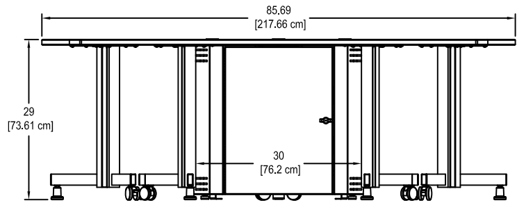
Asembled InVision Pod (without pedestal riser)
