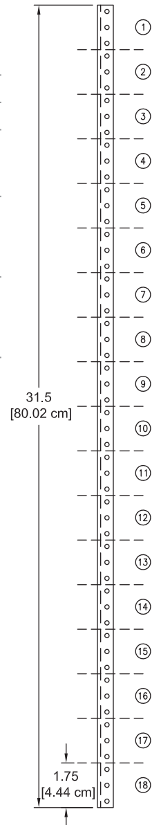
36RU available (18RU front and 18RU rear)
