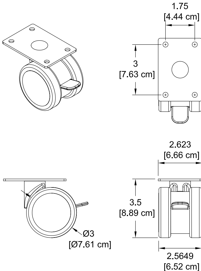
Twin-wheel casters
