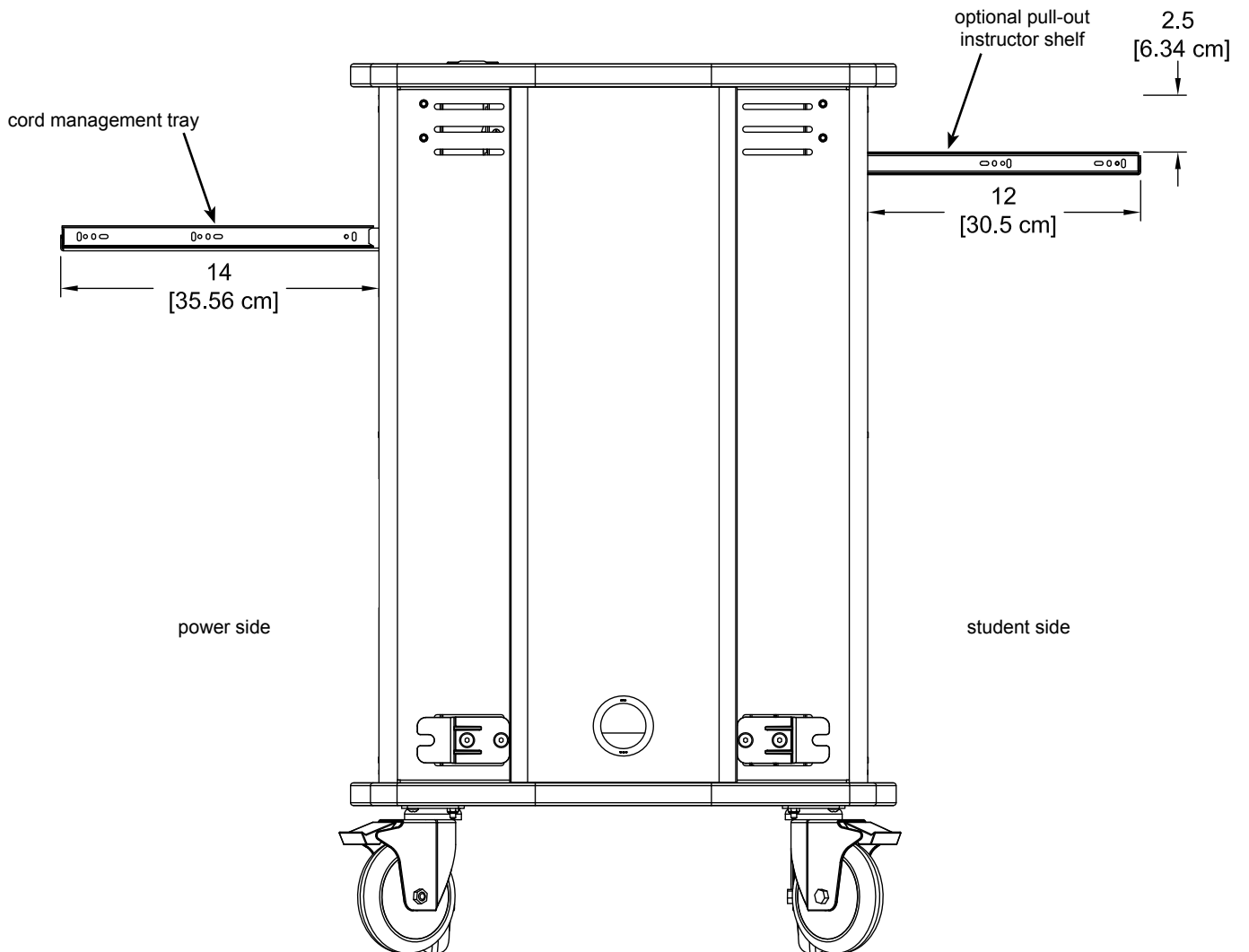
side view (shown with doors removed)
