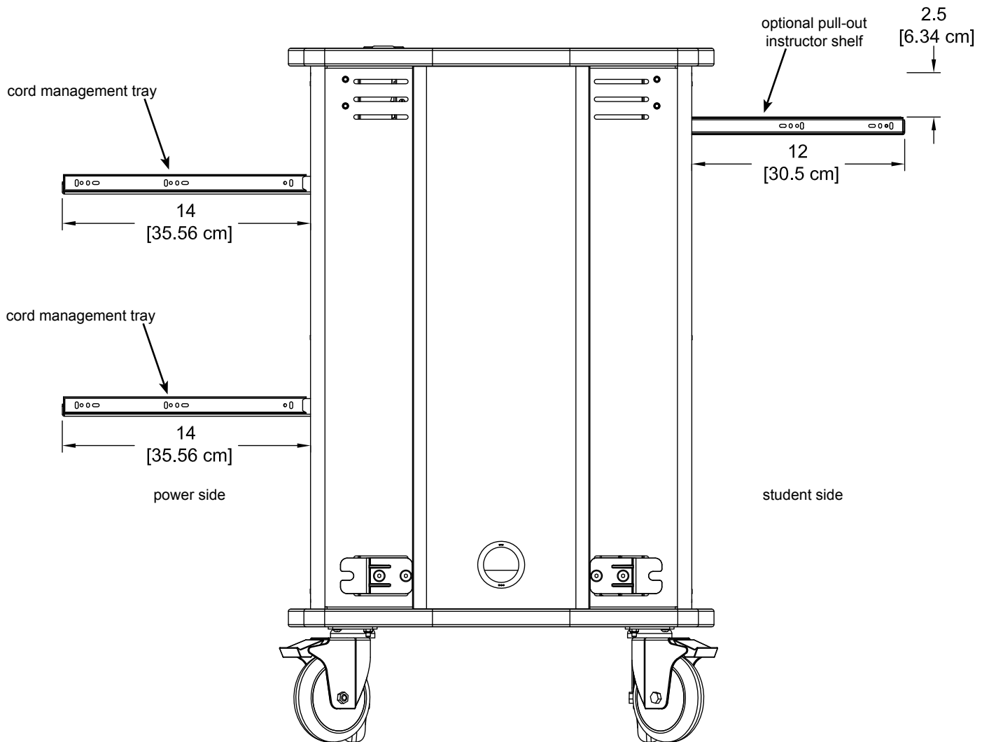
side view (shown with doors removed)
