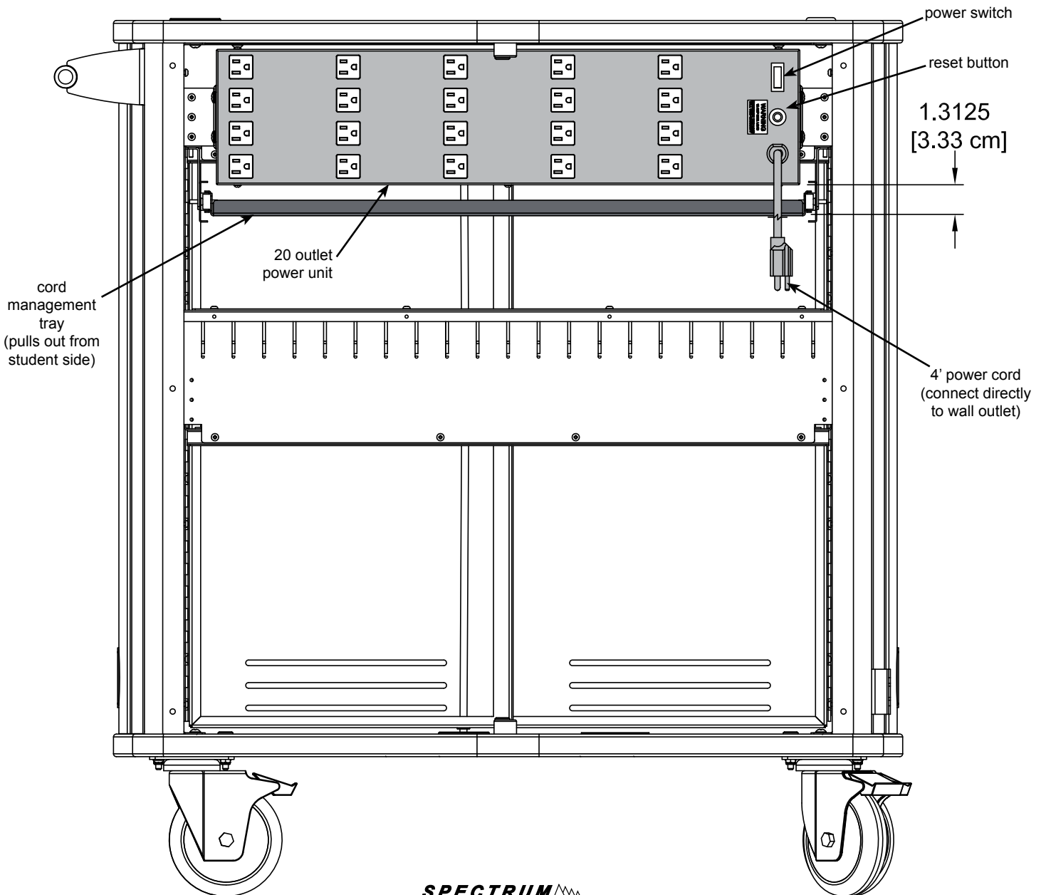
power side view (shown with doors removed)
