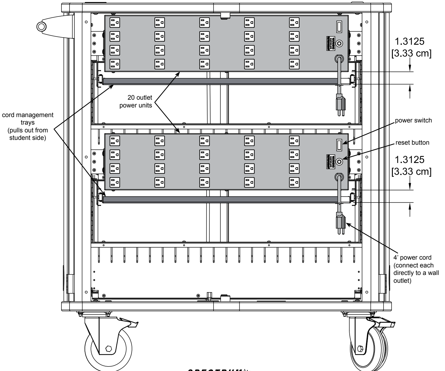
power side view (shown with doors removed)
