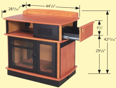
55251 CHBTK (overall dimensions)
