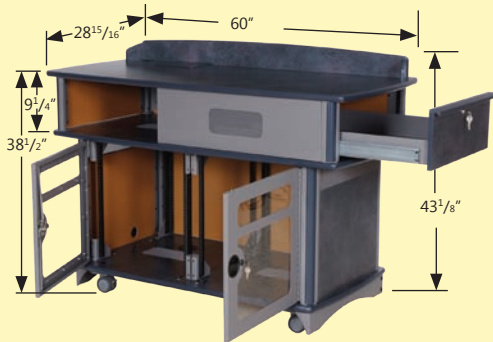
55245 IDTW (overall dimensions)
