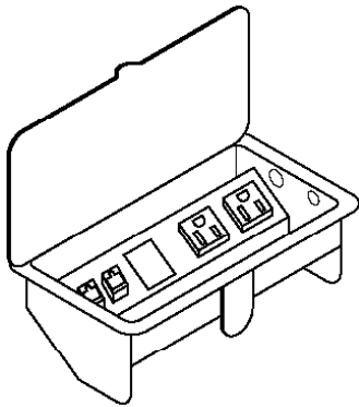
Power/Communication Module w/9' power cord, two outlets, two data jacks 7-1/8"W x 3-5/8"D 99002 (w/mic jack) 99003 (w/out mic jack)
