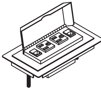
UL Listed Power/Communication Module w/9' power cord, two outlets, two data jacks, and adapter plate 7-1/8"W x 3-5/8"D x 3/4"H 99028
