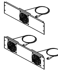
Cooling Fans (3RU) 19"W x 2"D x 5 1 / 4 "H Single Fan-97507 Double Fan-97506
