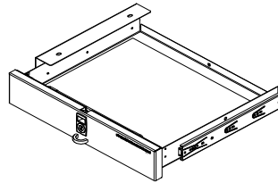
Keyboard Drawer w/ Flip-down front 18 3 / 4 "W x 16"D (Keyed the same as Doctorate drawer and front door) 55247
