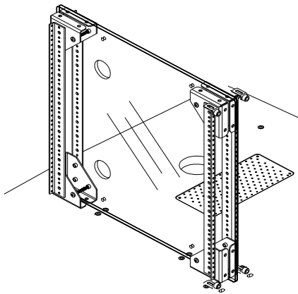
Clear Acrylic Security Panel 55246
