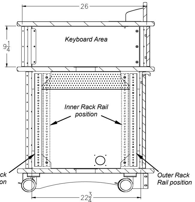
'A-A' Section View
