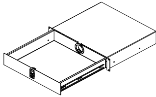
Locking Drawer (3RU) interior dims: 15 3 / 4 "W x 13 1 / 16 "D x 2 7 / 8 "H (25 lbs max load) 97514
